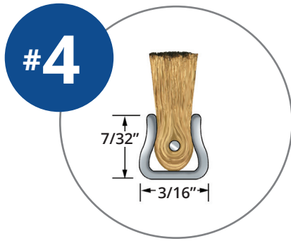
HOLDERS SHOWN FIT #4 STRIP BRUSHES
